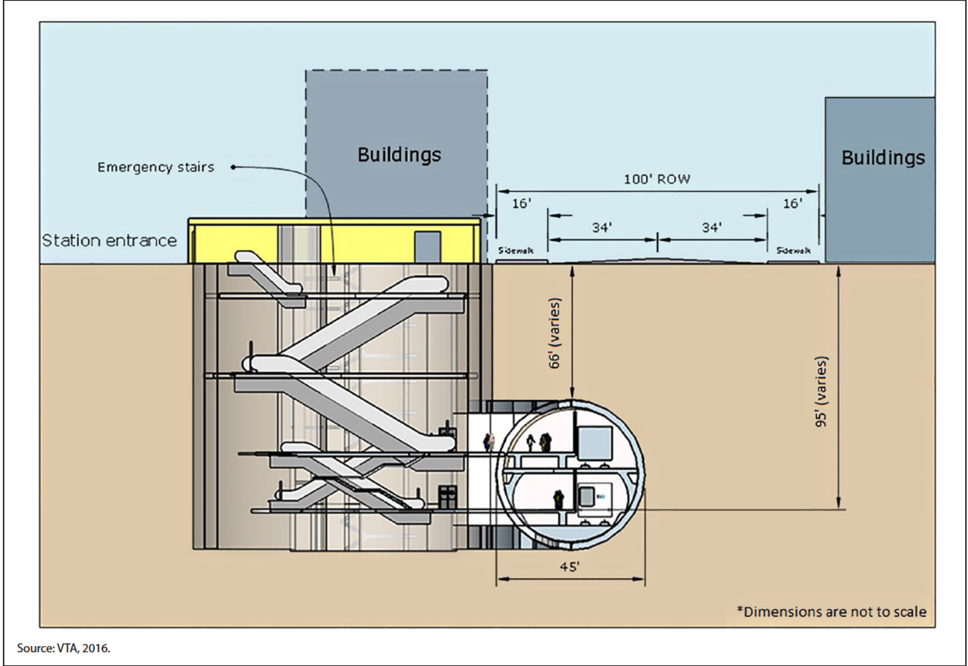
Figure 5-21 Example of Single-Bore Tunnel Station VTA's BART Silicon Valley-Phase II Extension Project
