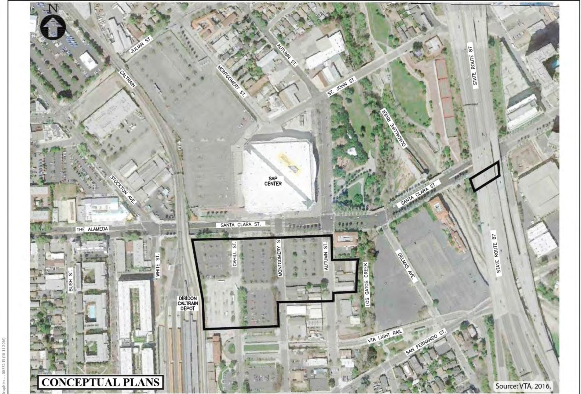
Figure 5-8 Proposed Diridon Station South Option Construction Staging Areas VTA's BART Silicon Valley–Phase II Extension Project
