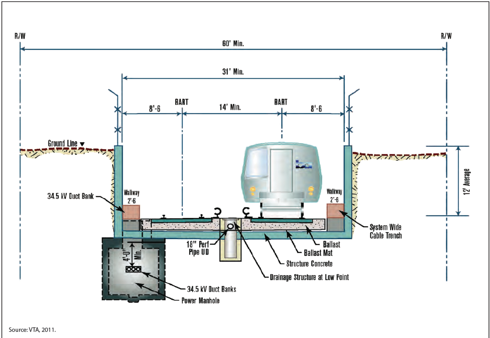
Figure 5-24 Retained Cut U-Wall
