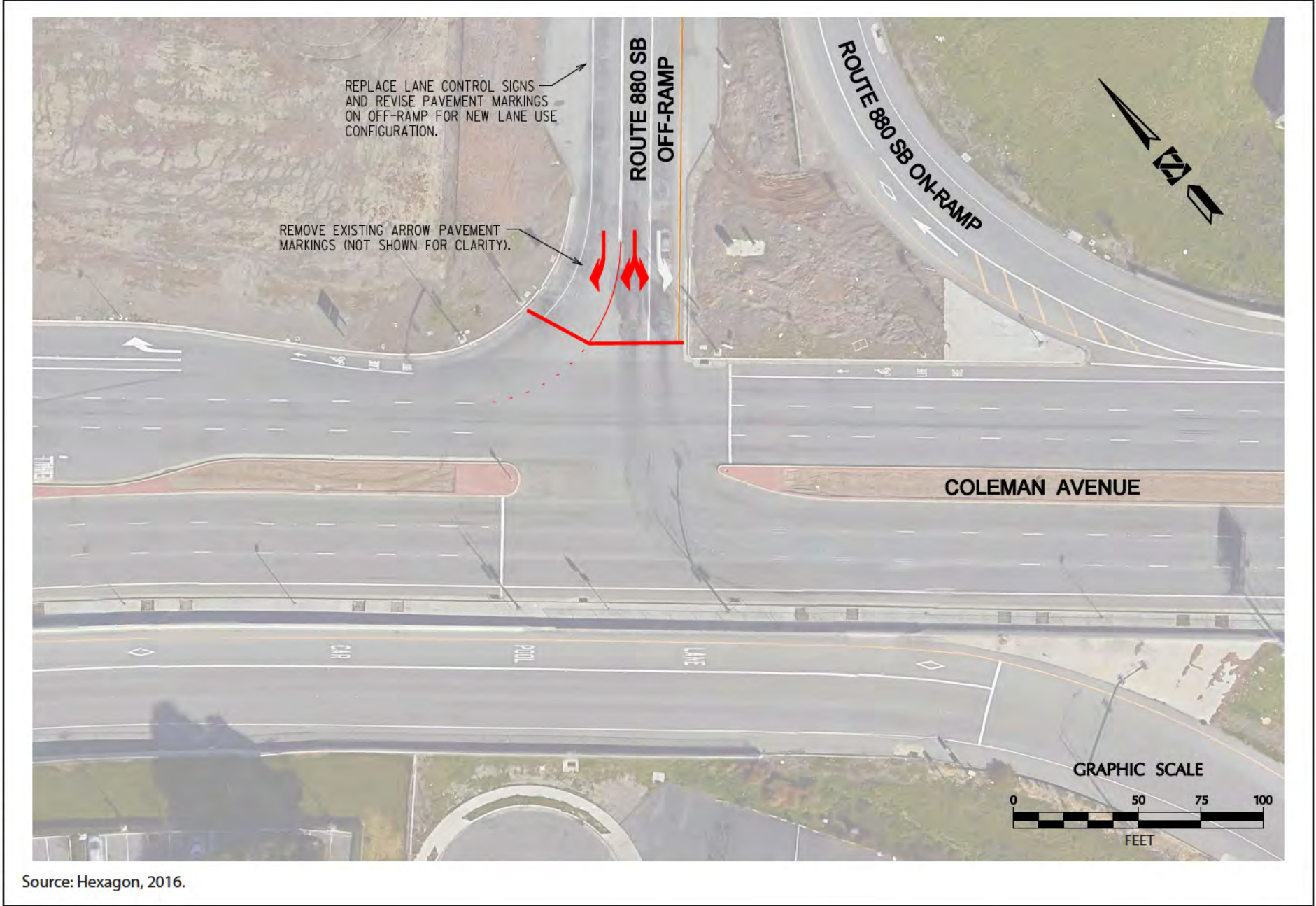
Figure 3-12 Proposed Mitigation for Coleman Avenue and I-880 Southbound Off-ramp VTA's BART Silicon Valley-Phase II Extension Project
