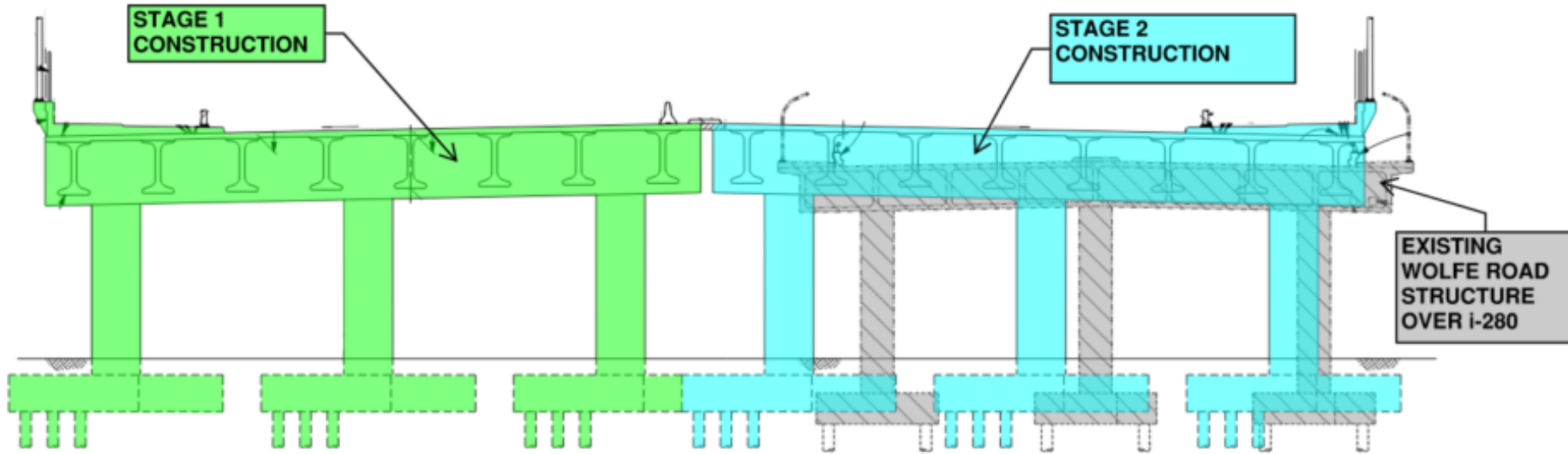
WOLF ROAD OVERCROSSING STRUCTURE TYPICAL SECTION CONSTRUCTION STAGES
