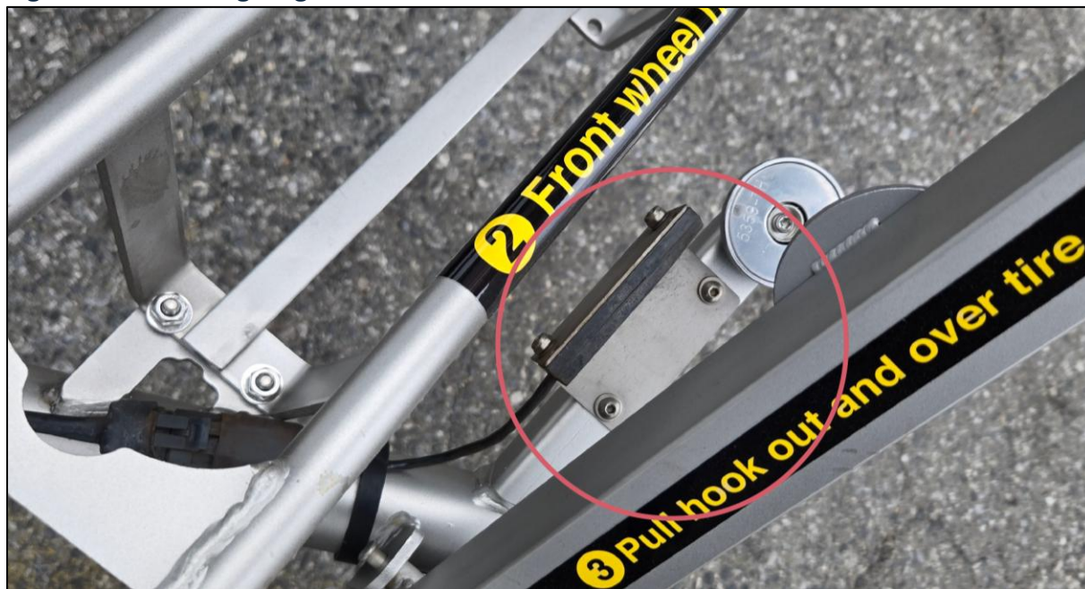
Figure 3-12. Missing Magnet on Bike Rack Retention Arm
